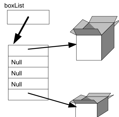
Model of an array of objects
