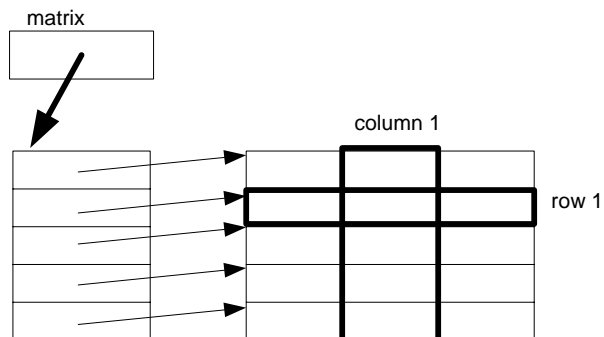
Model of an array of arrays
