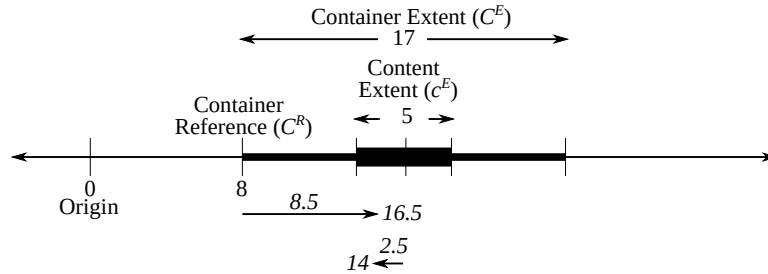
Figure 21.1: Centering in One Dimension
