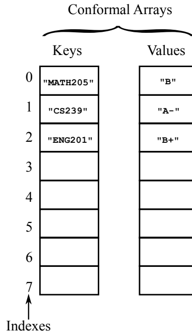
Figure 17.2: An Example of Keys and Values in Conformal Arrays
