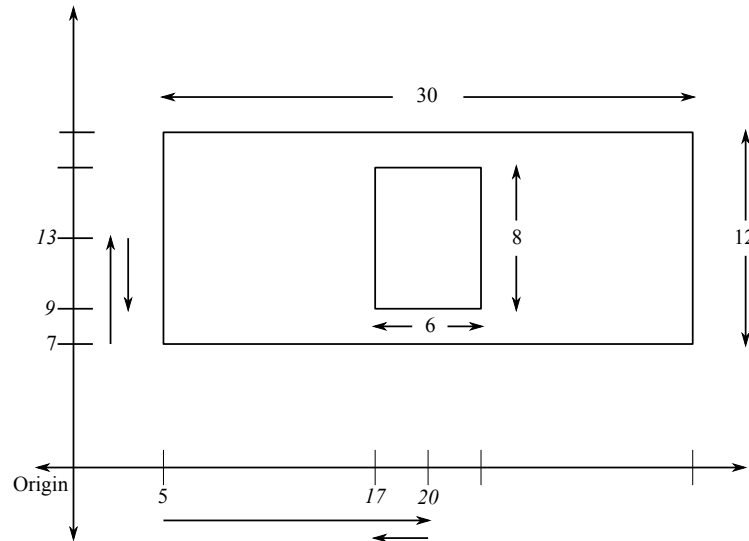
Figure 21.2: Centering in Two Dimensions
