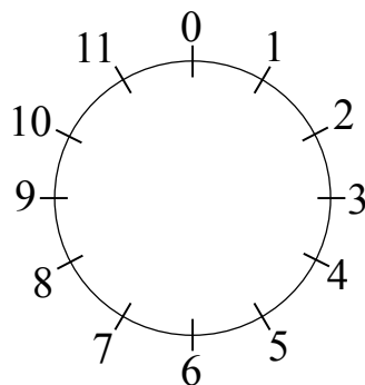
Figure 4.4: Numbers on a Circle
