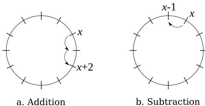
Figure 4.5: Addition and Subtraction on a Circle
