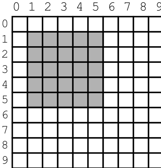
Figure 20.2: A 5 \times 5 Neighborhood around Element (3,3)
