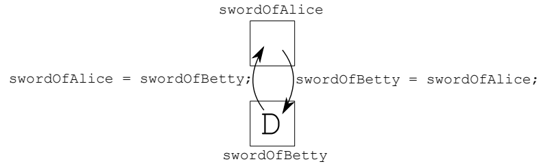
Figure 1.2: A Defective Swapping Algorithm
