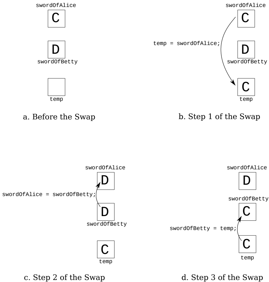
Figure 1.4: Steps in a Swap
