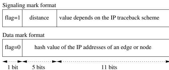
Figure 4. Mark format for signaling and data subchannels
