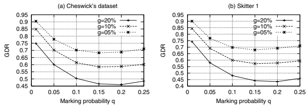
Figure 9. GDR (Good Drop Ratio)
