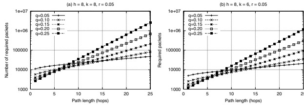
Figure 5. Expected number of marks (Y-axis) needed for reconstructing a path of certain length (X-axis)
