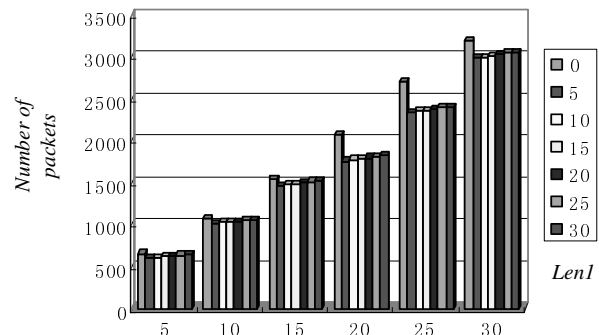
Figure 9: Bar chart representation of minimum number of packets needed for attack paths reconstruction ( q = 0.01 ).
